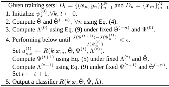
Figure 1: Algorithm of learning model parameters in proposed method with naive Bayes model.
